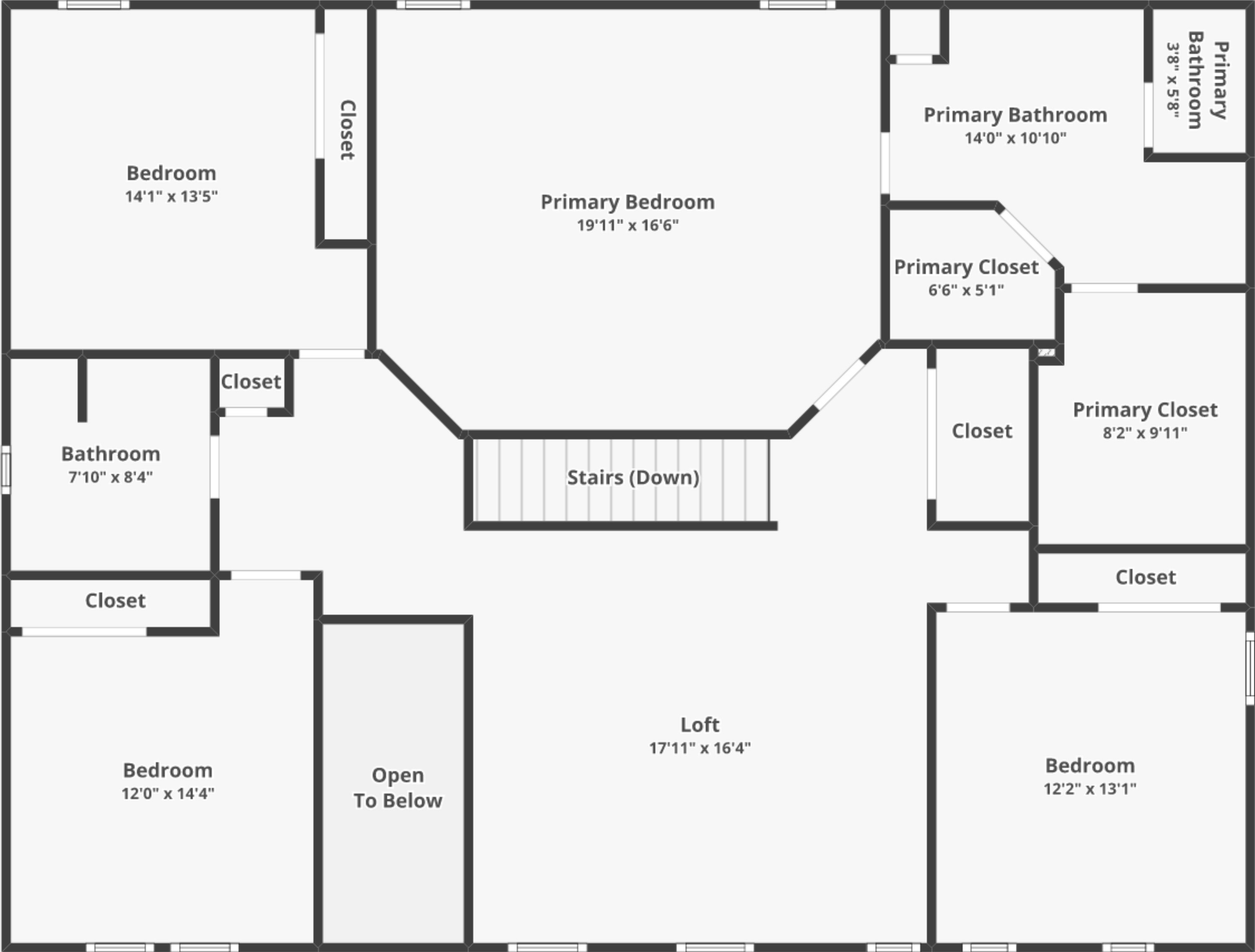
FLOOR 2
